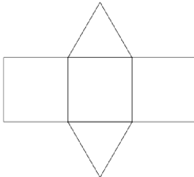
Triangular Prism
