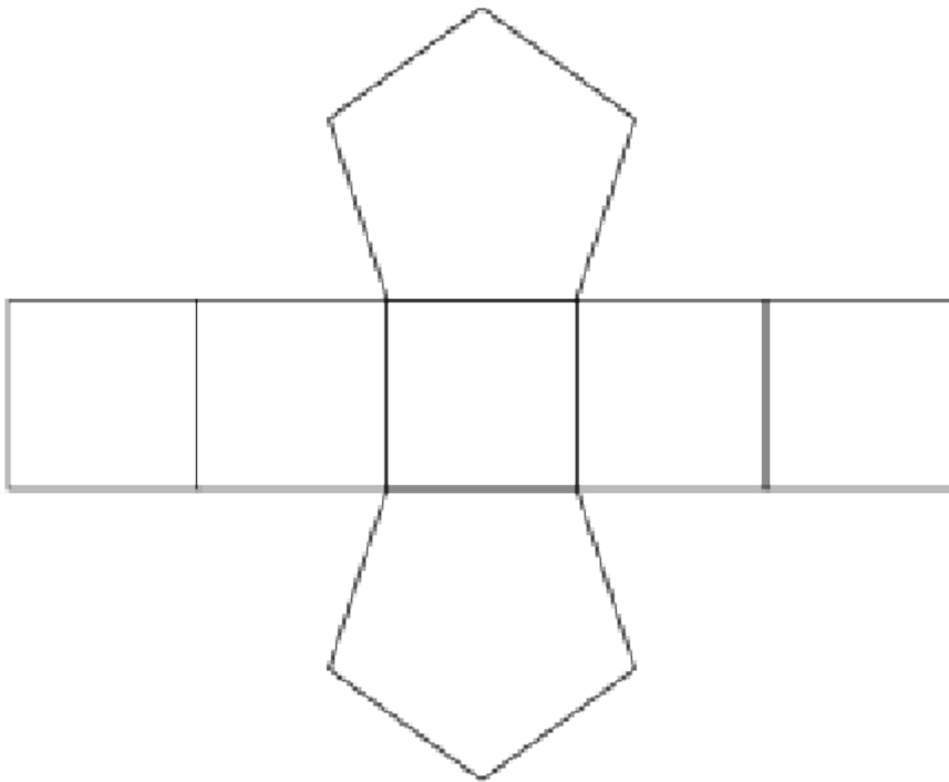
Pentagonal Prism
