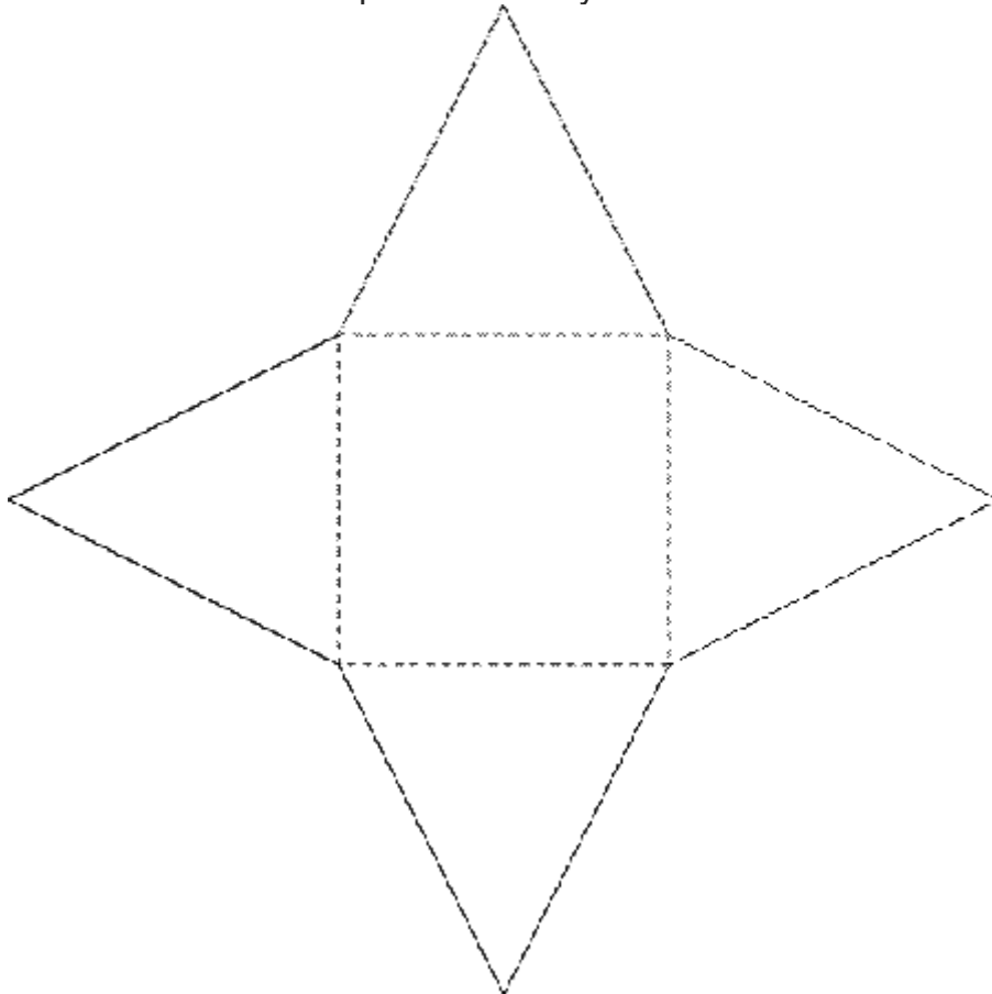
Square-based Pyramid
