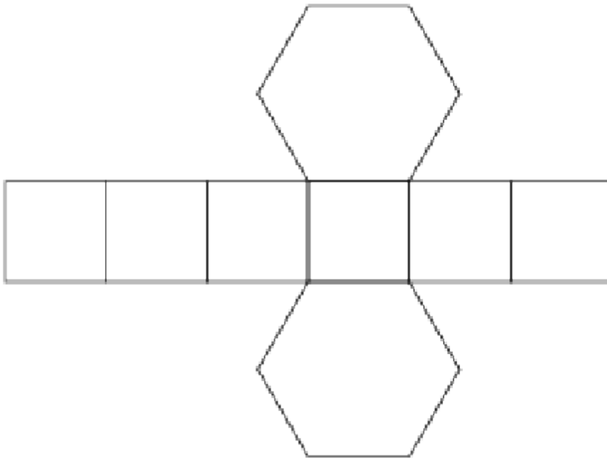
Hexagonal Prism
