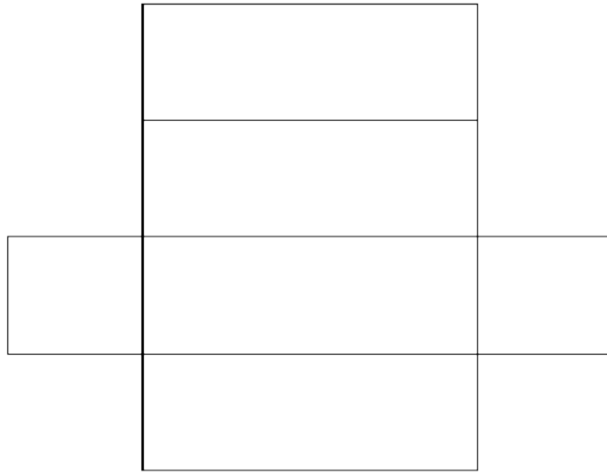
Rectangular Prism
